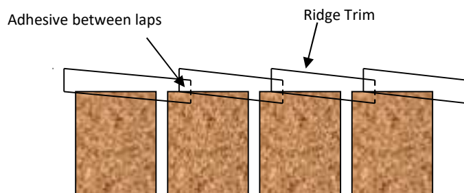
Ridge Detail
